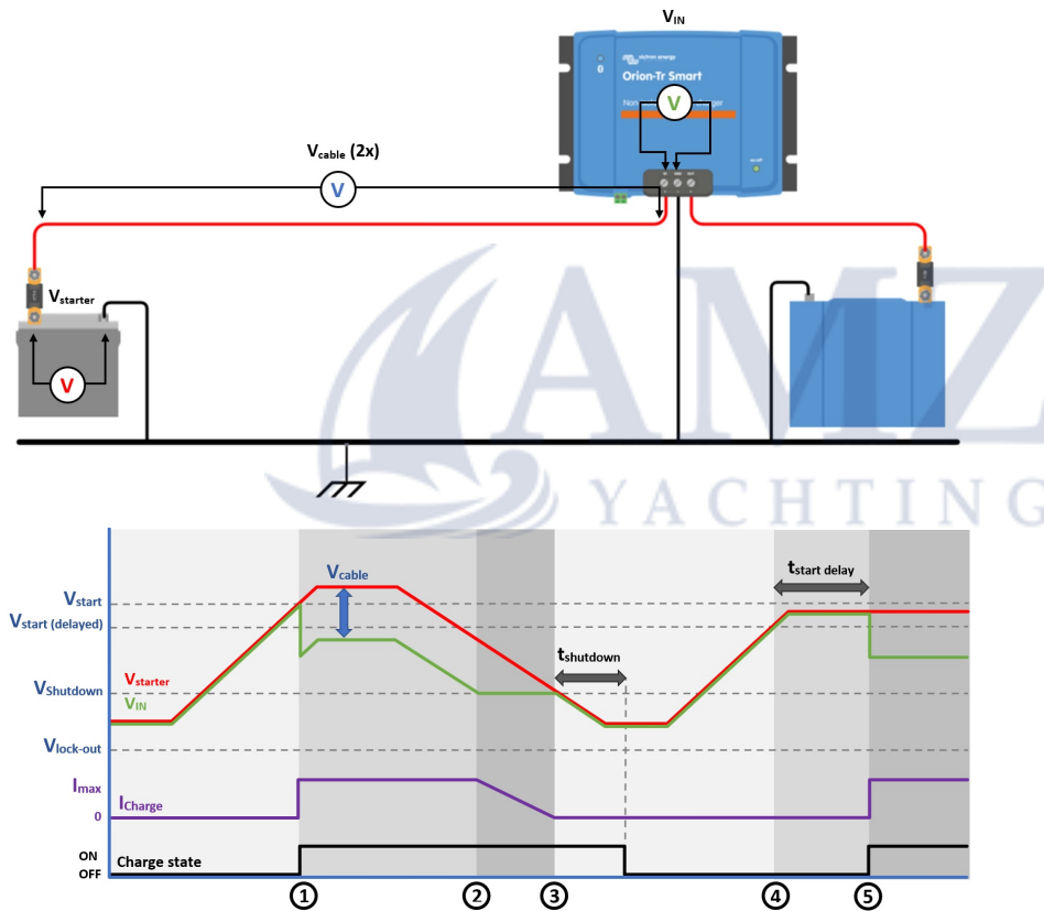
Figure 8: Engine shutdown detection sequence
